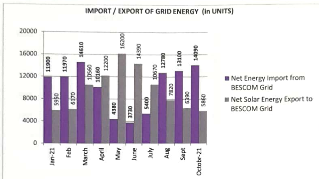
e) Graph - Month wise Import / Export of Grid Energy JAN - OCT-21
